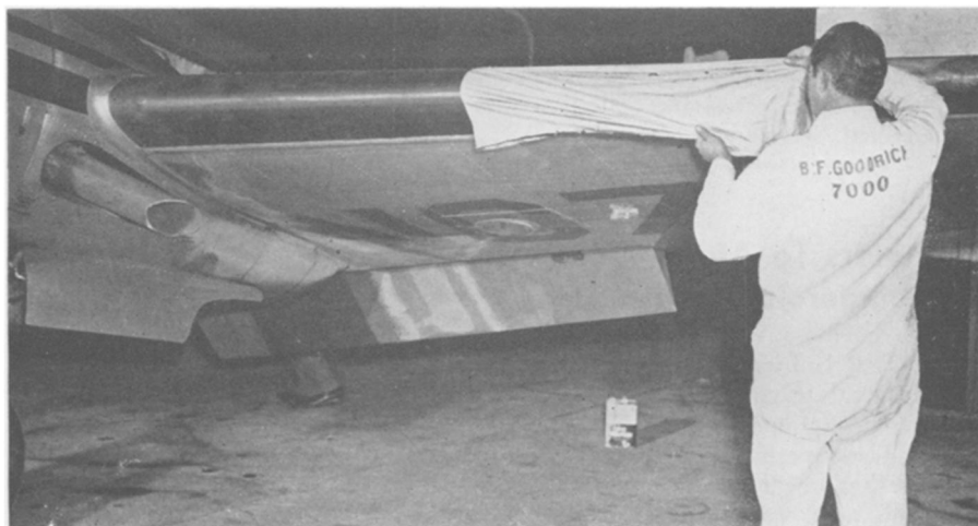
FILM STRIPPING —A thin film is applied on airplane de-icers to protect the rubber from hot weather. At the end of the season it can be stripped off as shown.
